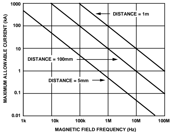
Figure 14. Maximum Allowable Current for Various Current-to-ADuM320x Spacing
